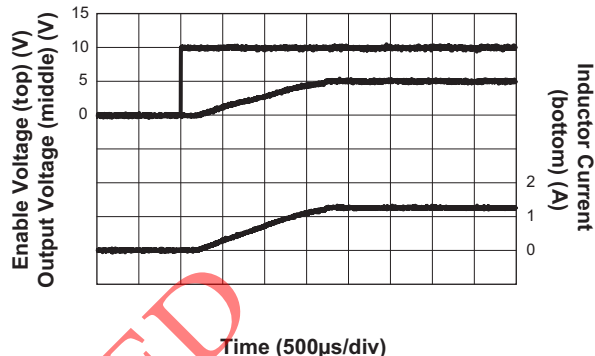
Step-Down Converter Soft Start (V_{IN} = 12V; V_{EN} = 10V; V_{OUT} = 5V; I_{OUT} = 1.2A)
