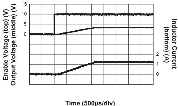
Step-Down Converter Soft Start (V_{IN} = 12V; V_{EN} = 10V; V_{OUT} = 3.3V; I_{OUT} = 1.2A)
