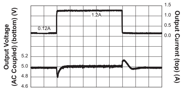
Time (100µs/div)
