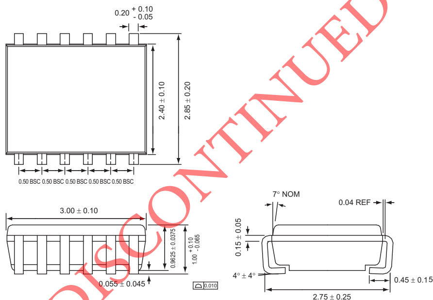
TSOPJW-12
